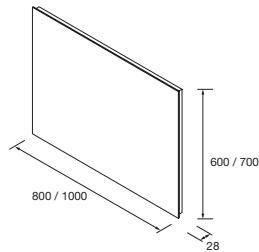
Espejo BLOCK 1000 horizontal vertical luz led (25 W-5700°K) IP44 - 700 x 1000 mm 105598
